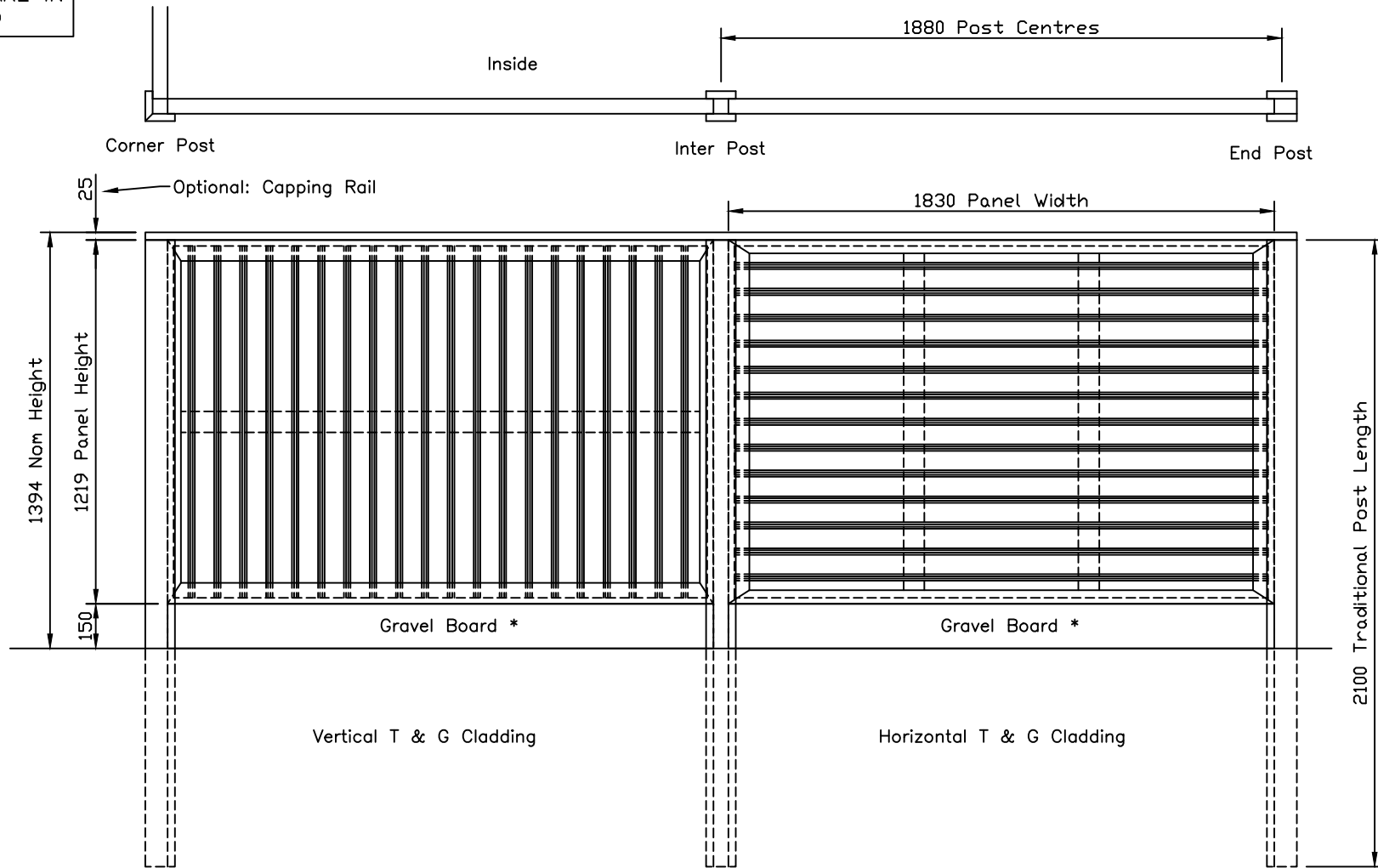
Tongue & Groove Fencing with Slotted Posts
