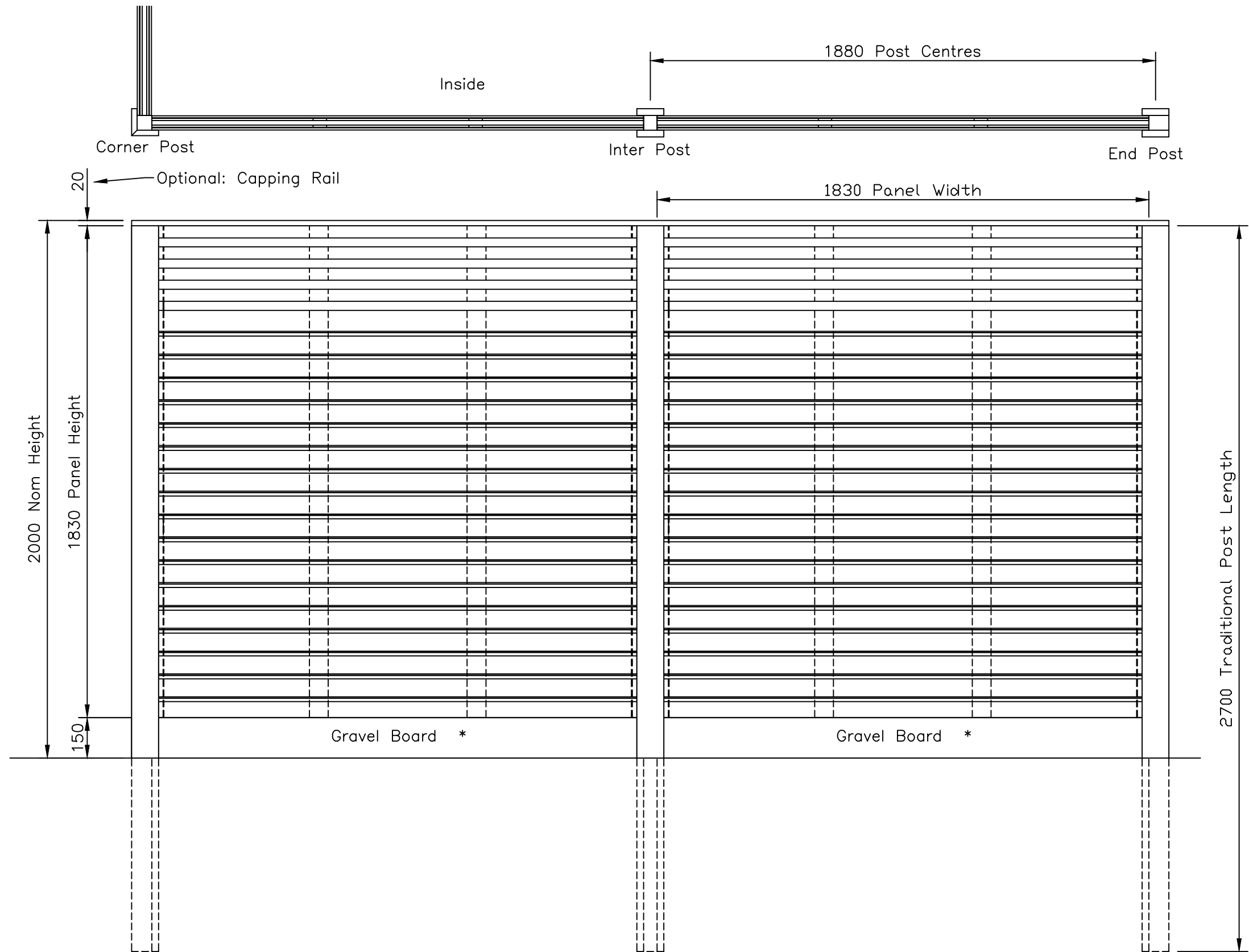
Canterbury Combi Fencing with Slotted Posts
