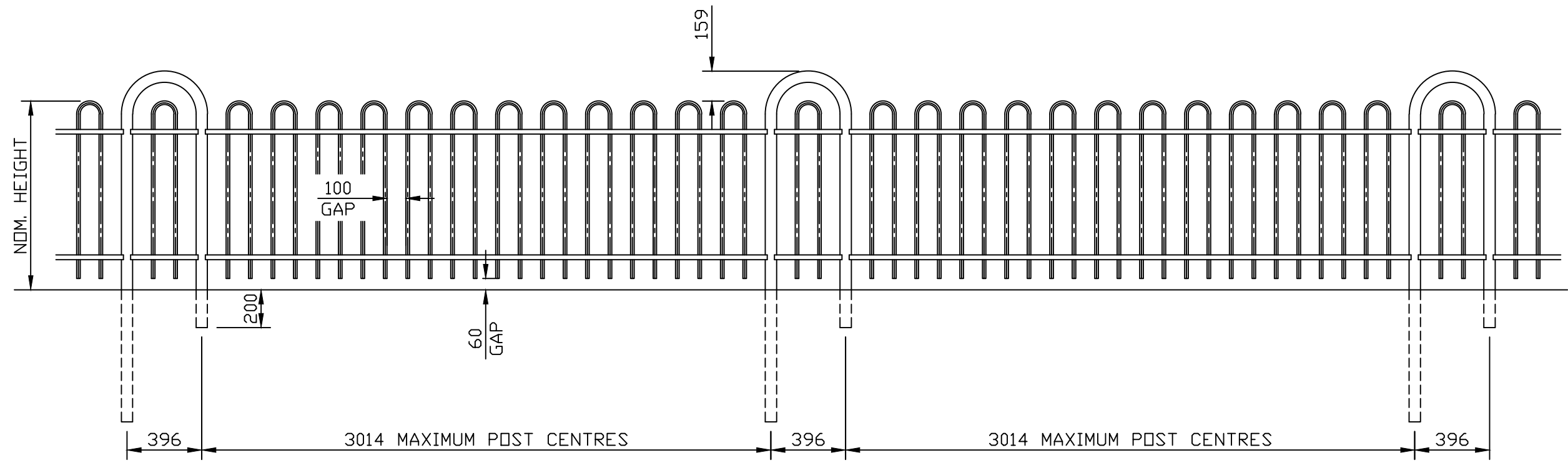
STANDARD BOWTOP PANELS WITH FEATURE POSTS
