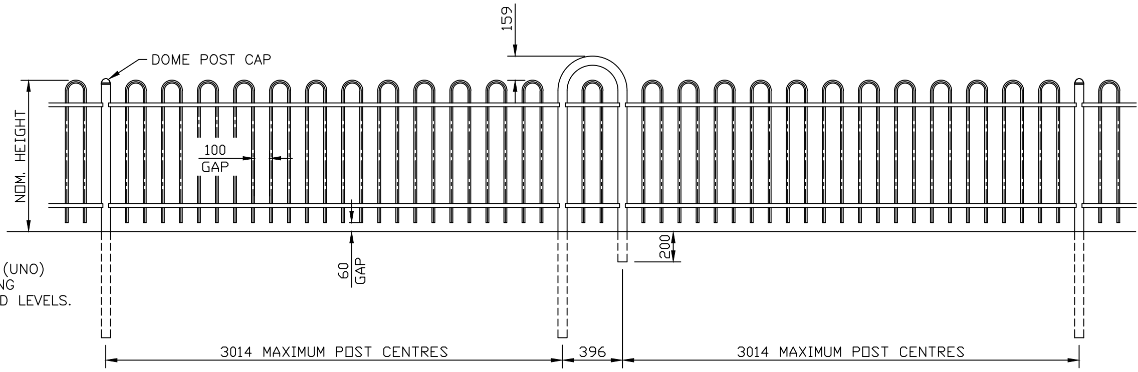
STANDARD BOWTOP PANEL & POSTS WITH OCCASIONAL FEATURE POST
