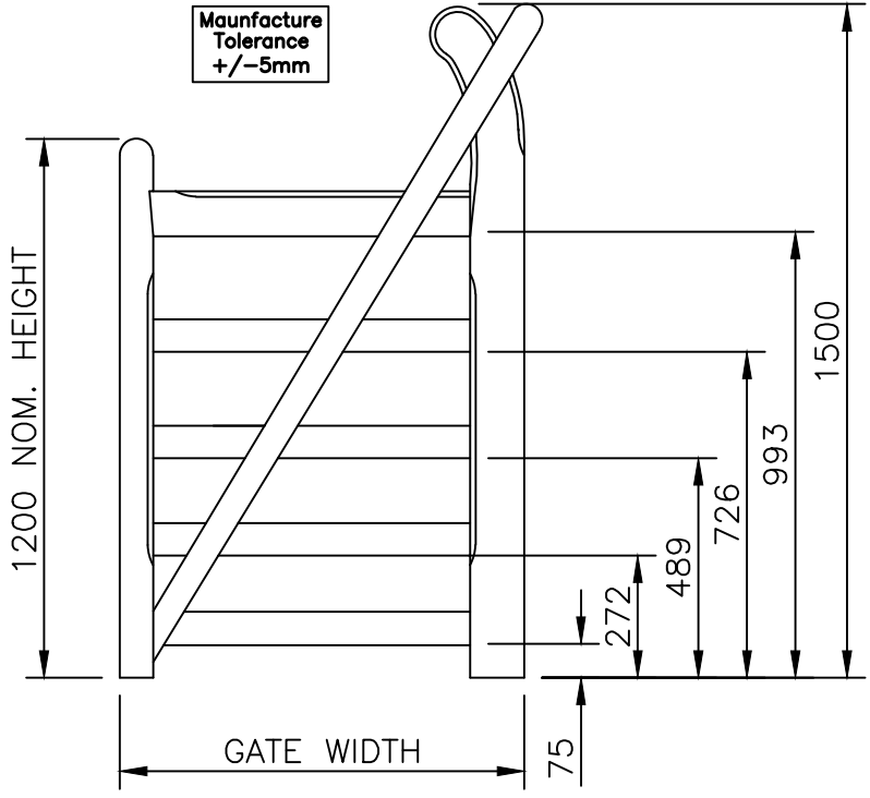
VIEWED FROM OUTSIDE GATE RIGHT HAND HANGING. PLEASE STATE HAND REQUIRED.
