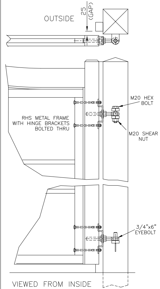
TIMBER CLAD POST OPTION (17mm THK CLADDING)
