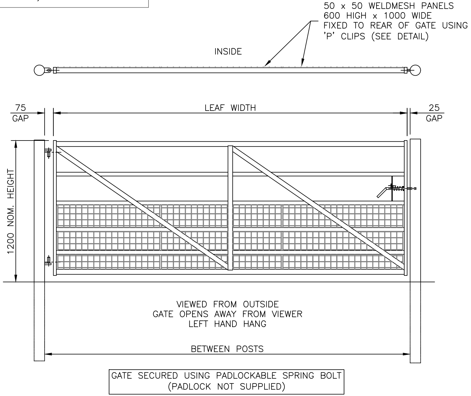
STANDARD SINGLE METAL FIELD GATE – WELDMESH CLAD (POSTS HUNG IN LINE)
