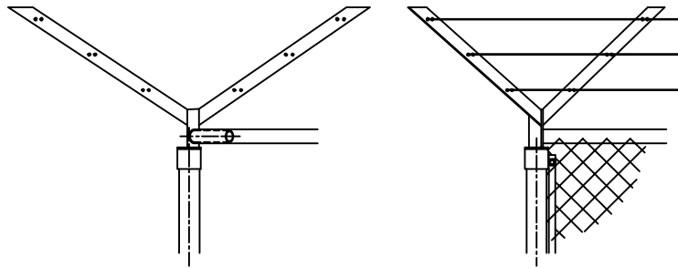
'Y' CORNER
