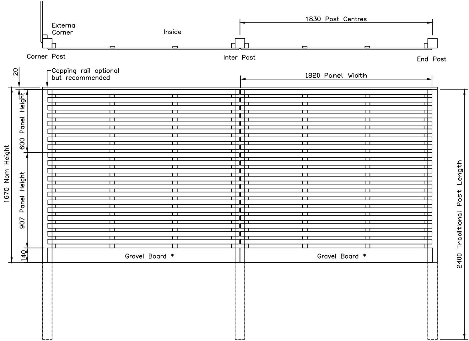
Metro Fencing with Heavy Duty Panel Posts Viewed from Outside
