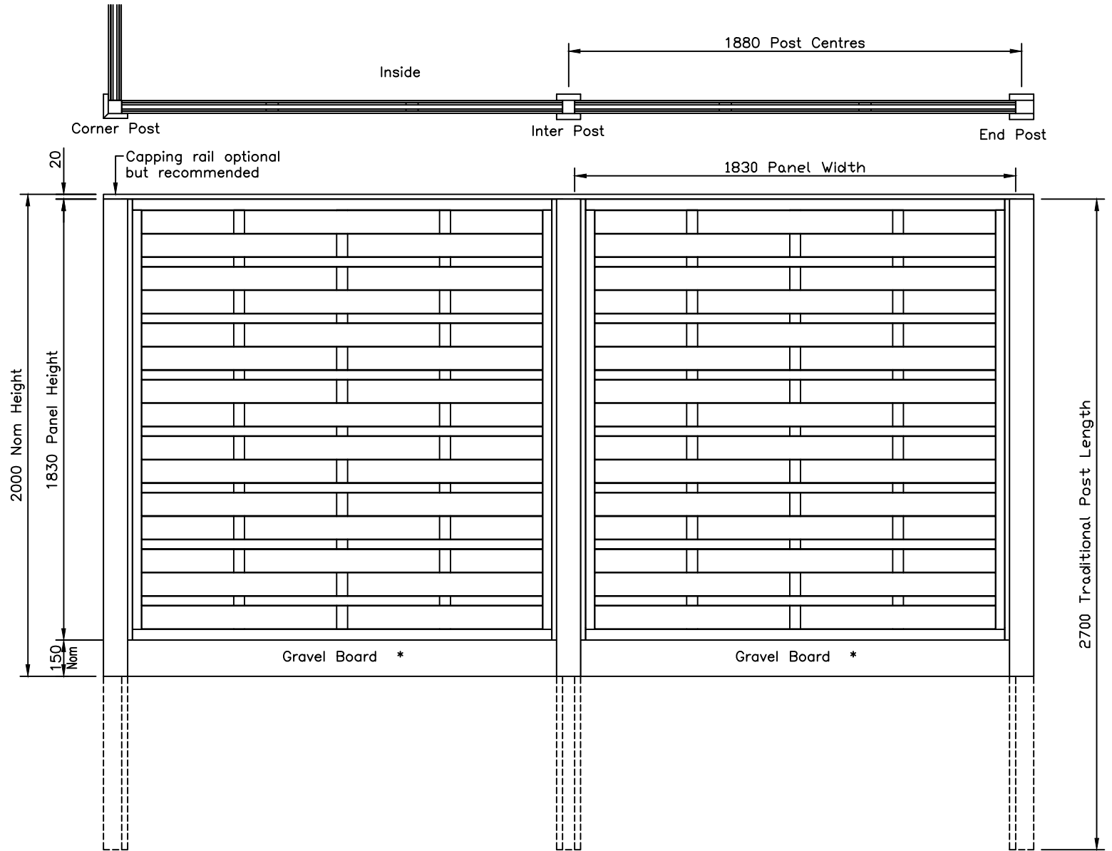
Aran Fencing with Slotted Posts Viewed from Outside
