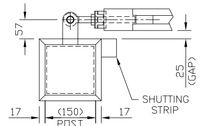
TIMBER CLAD POST OPTION (17mm THK CLADDING)
