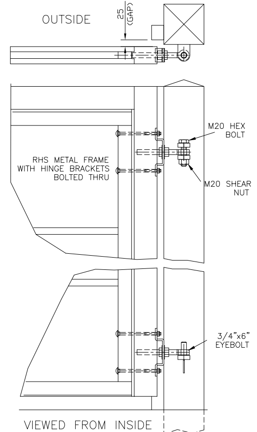
TIMBER CLAD POST OPTION (17mm THK CLADDING)
