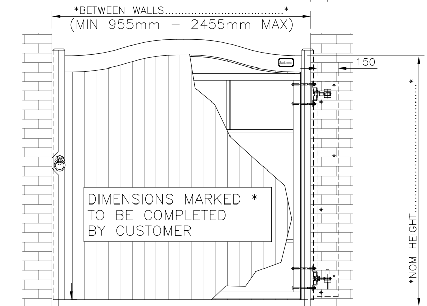
50 GAP VIEWED FROM OUTSIDE GATE OPENS AWAY FROM VIEWER RIGHT HAND HANG (AS DRAWN) OPTION 'B'
