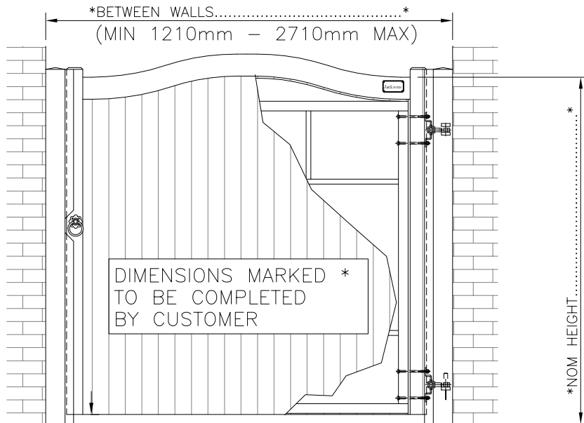
50 GAP VIEWED FROM OUTSIDE GATE OPENS AWAY FROM VIEWER RIGHT HAND HANG (AS DRAWN) OPTION 'A'
