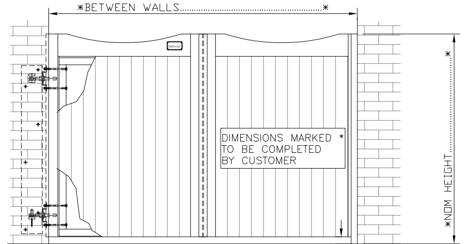
VIEWED FROM OUSTIDE GATES OPEN AWAY FROM VIEWER
