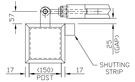
TIMBER CLAD POST OPTION (17mm THK CLADDING)
