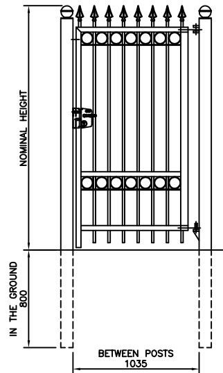
VIEWED FROM OUTSIDE GATES OPEN AWAY FROM VIEWER
