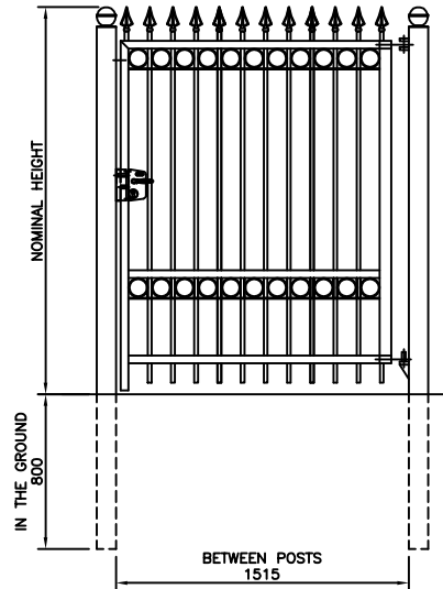
VIEWED FROM OUTSIDE GATES OPEN AWAY FROM VIEWER
