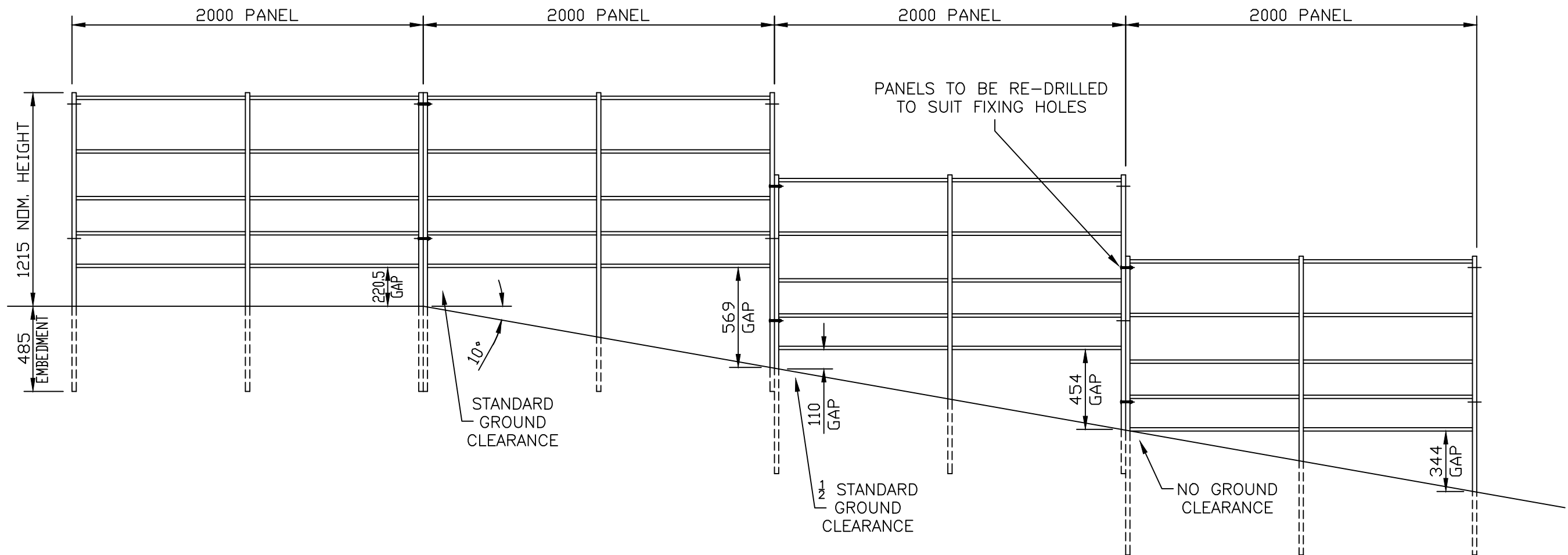
ESTATE FENCE – STEPPED EXAMPLE TO SUIT 10° SLOPE
